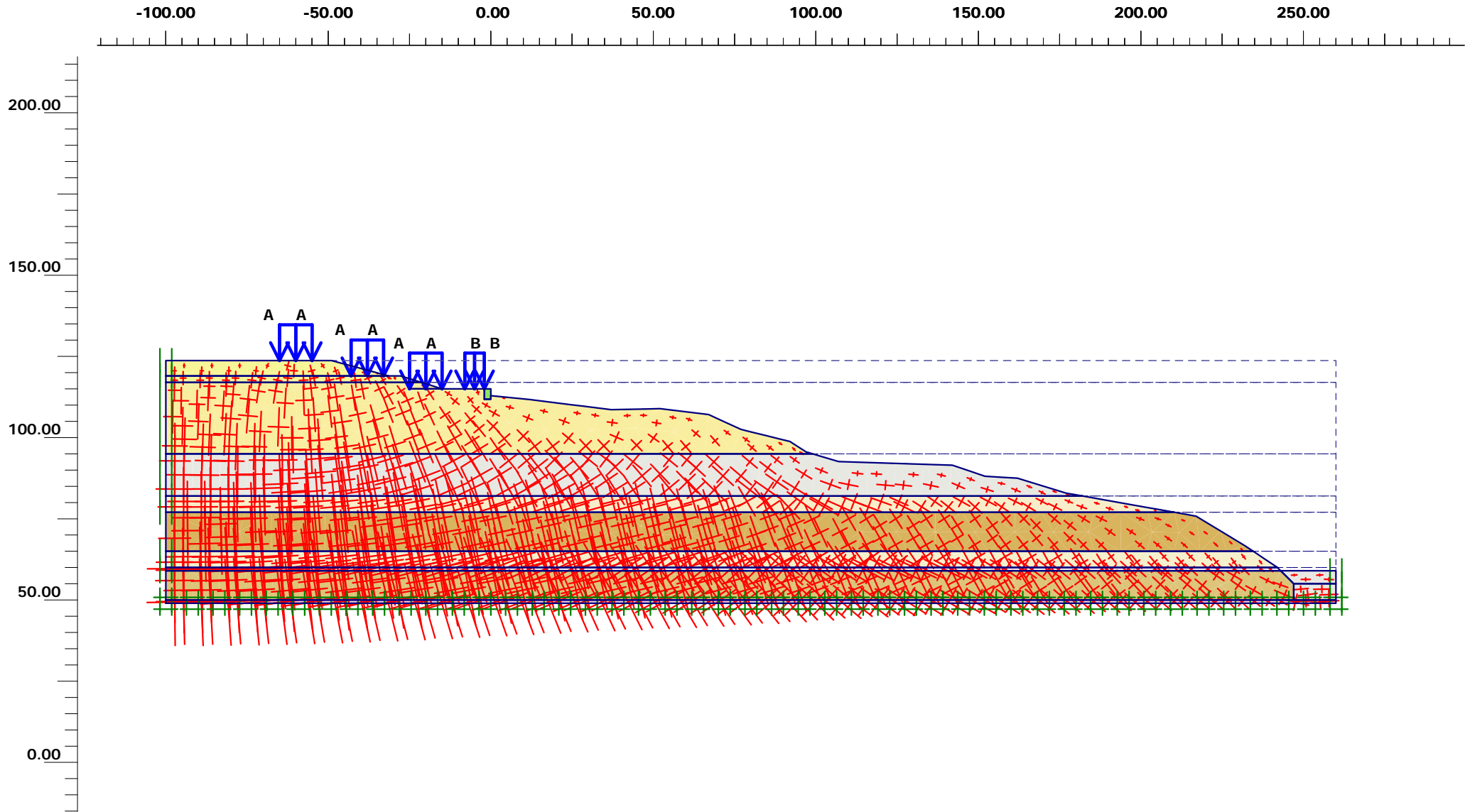
Effective stresses Extreme effective principal stress -670,21 kN/m 2
